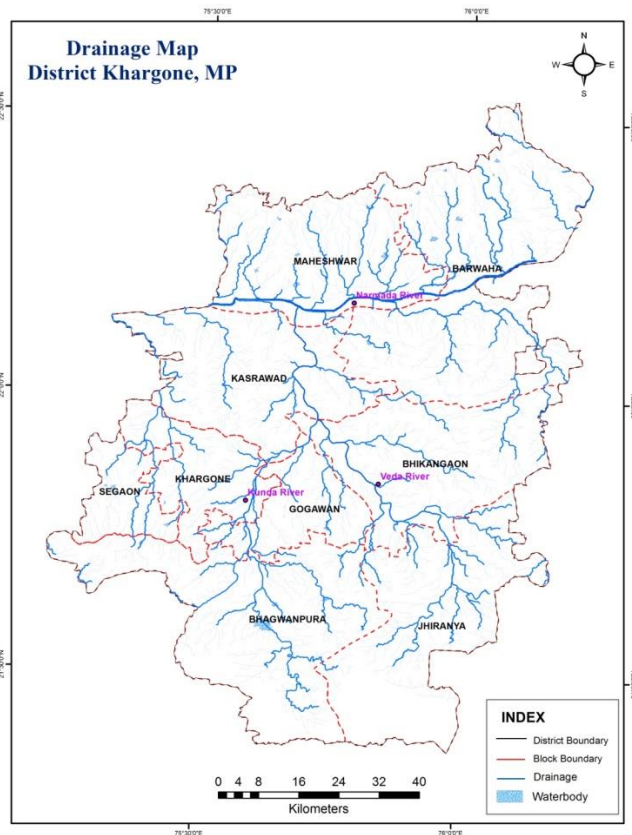
Figure 4: Drainage Map of Khargone district
